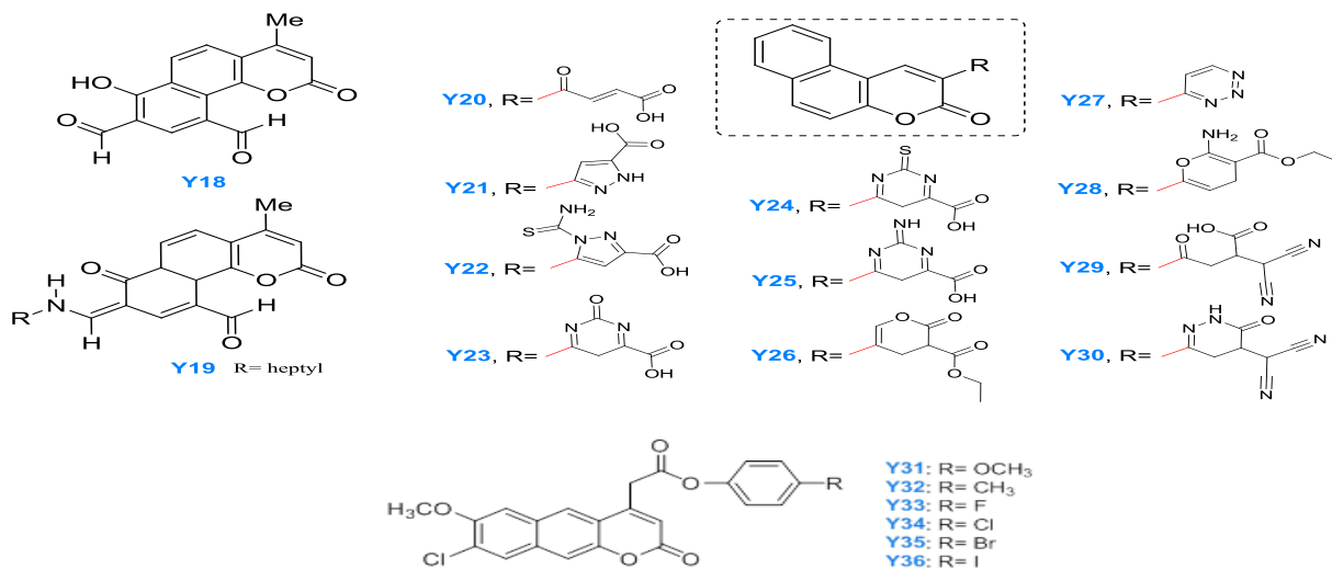
Figure 5: As oxidative inhibitors, Sashidhara and colleagues created benzo[ h ]coumarins ( Y18 and Y19 ). Salem and colleagues synthesized benzo[ f ]coumarins ( Y20–Y30 ) as free radical quenchers. Furthermore, Waheed and Mustafa's benzo[ g ]coumarin-related compounds ( Y31–Y36 ) have antioxidant properties.
