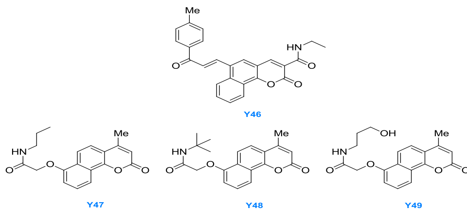
Figure 8: Sashidhara and colleagues synthesized a benzo[ h ]coumarin-derived compound ( Y46 ) with antithrombotic activity. Sashidhara and colleagues developed antithrombotic benzo[ h ]coumarins ( Y47–Y49 ).
